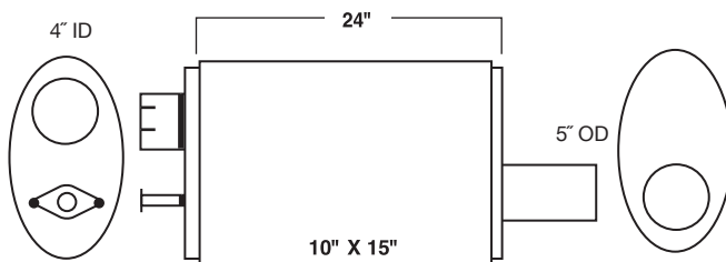
MODEL: CAT 631D
