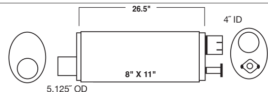
MODEL: CAT 927B 9S7079
