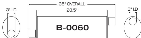
1996-1998 CHEVROLET/G.M.C. C1500/2500, K1500/2500
