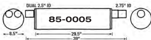
FORD MED. DUTY 370-429 C.I.
