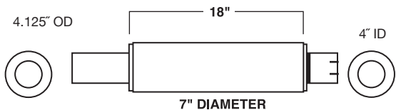
MODEL: CAT 518 9S9328
