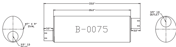
1992-1996 DODGE RAM, DAKOTA
