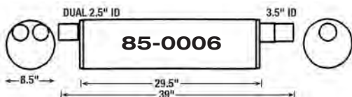
FORD MED. DUTY 370-429 C.I. "HIGH FLOW"
