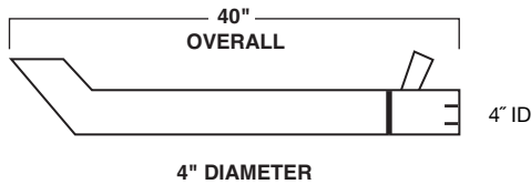
MODEL: CAT D6H STACK 7W5838
