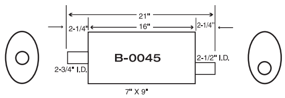
1992-1996 DODGE RAM, DAKOTA
