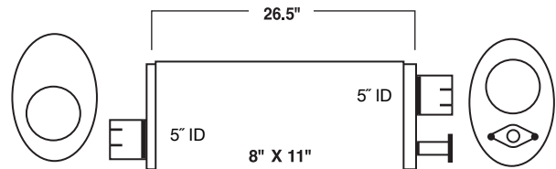
MODEL: CAT 980B, 330JB 7N3235
