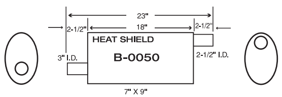
1992-1995 CHEVROLET/G.M.C. ASTRO/SAFARI VAN
