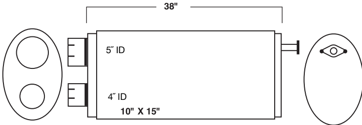
MODEL: CAT 627B 6N4183
