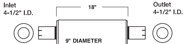
MODEL: CAT 977 LOADER 7S6741
