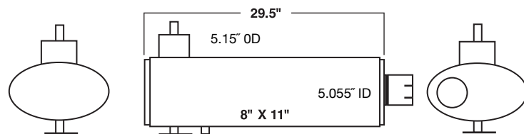
MODEL: CAT D8K 6N5437
