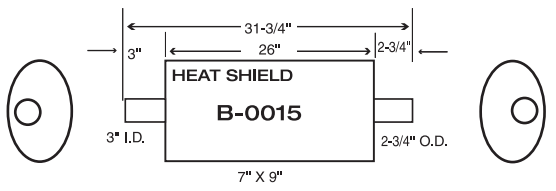
1994-1995 CHEVROLET/G.M.C. C1500/2500, K1500/2500, SUBURBAN, 2WD with 3" INLET
