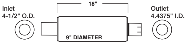
MODEL: CAT 966 LOADER 7S8443
