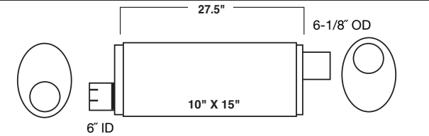
MODEL: CAT 988, 824B, 826B 8S6443
