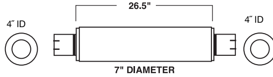
MODEL: CAT 627B 9S8069
