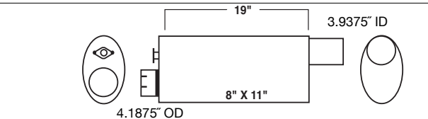
MODEL: CAT 140G 8N5565
