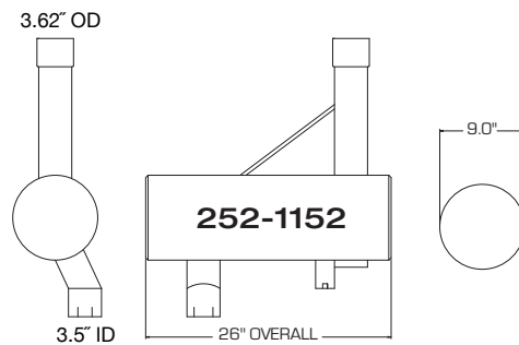
Model : D6M CAT
