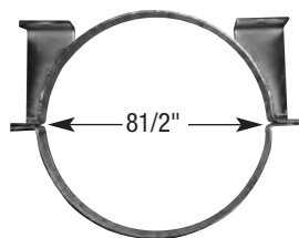
MUFFLER HANGER TP85MH SEE PAGE T 30
